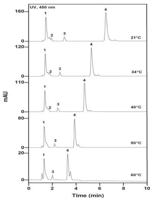
Fig 3 Internal standards of different carotenoids in different temperatures
