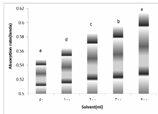
Fig 1 Absorbance of different volumes of Ethanol in boiling point
