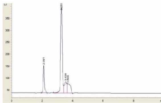
Fig 2 Retention Time (RT) of standard β- carotene solution
